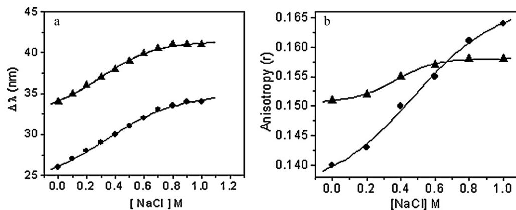
Fig. 6. Plots of (a) shift of emission maximum ( \Delta\lambda ) of AN versus [\text{NaCl}] and (b) anisotropy ( r ) of DPH versus [\text{NaCl}] in 0.25 g/L of the copolymers, (●) SAVal-DA(0.09) and (▲) SAVal-DA(0.16).
