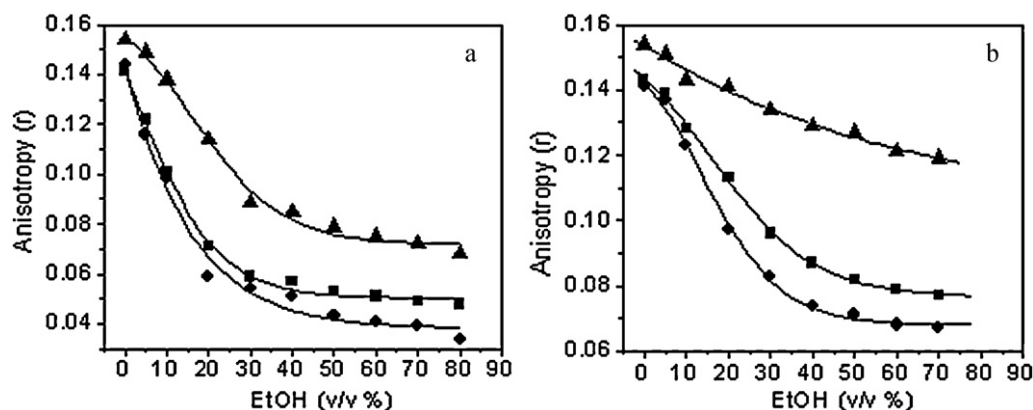
Fig. 5. Plots of fluorescence anisotropy ( r ) of DPH as a function of [\text{EtOH}] (v/v %) for (a) 0.25 g/L and (b) 1.0 g/L, (●) SAVal-DA(0.09), (■) SAVal-OA(0.16), and (▲) SAVal-DA(0.16) copolymers.
